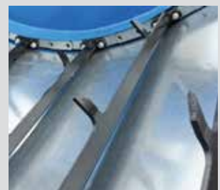
3 and 4 tooth slats rip tough, uneven bales
